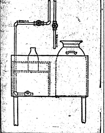
Sink Arranged for Pasteurization of Milk.
